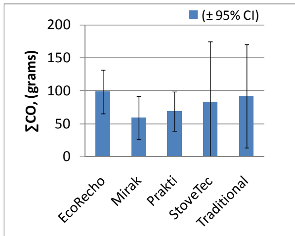
Fig. 10: Total CO Emissions for Simmer Phase. Error bars are \pm 95\% confidence intervals.
